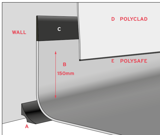
Figure 2 Overlap installation method
