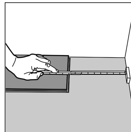
Figure 49 Last plank, first row
